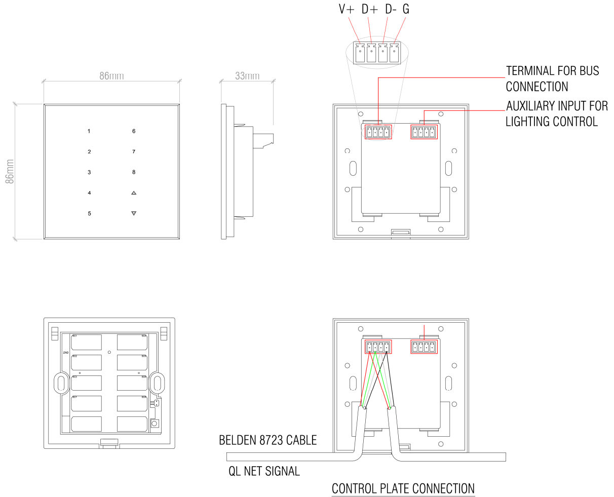
Fig 1. Control Plate Details
