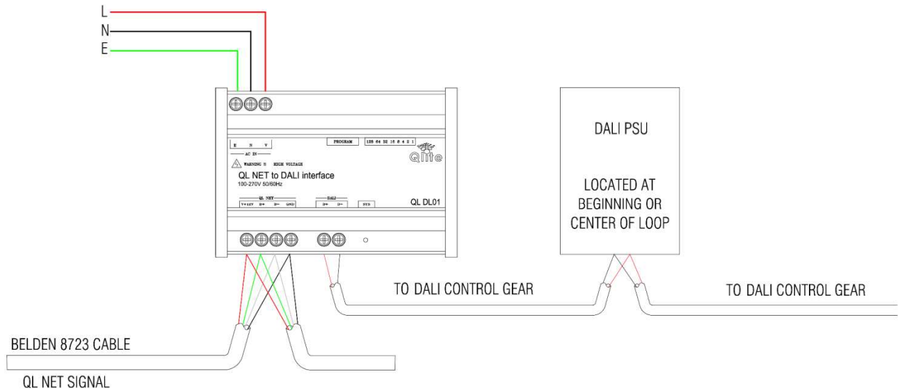
Fig 2. Module Connections
