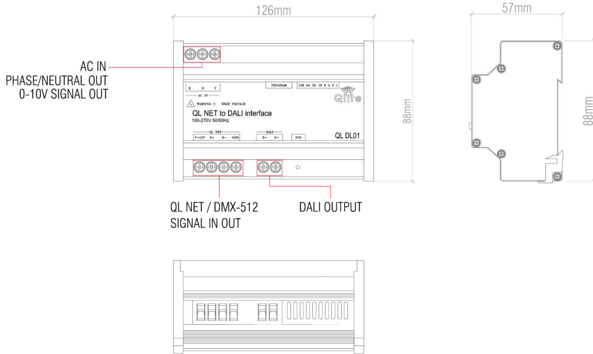
Fig 1. Module Details
