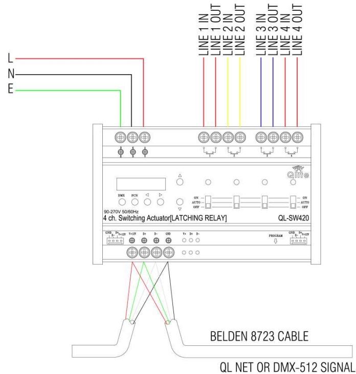
Fig 1. Module Details
