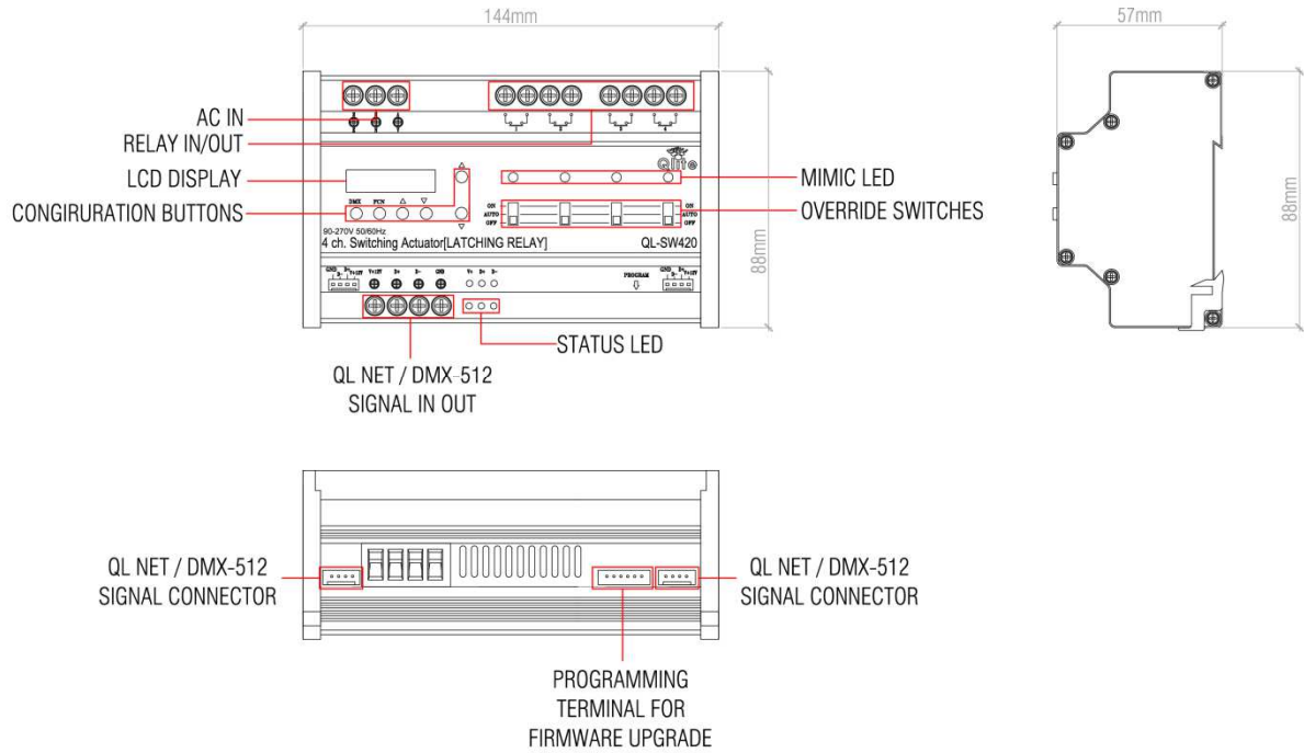
Fig 1. Module Details
