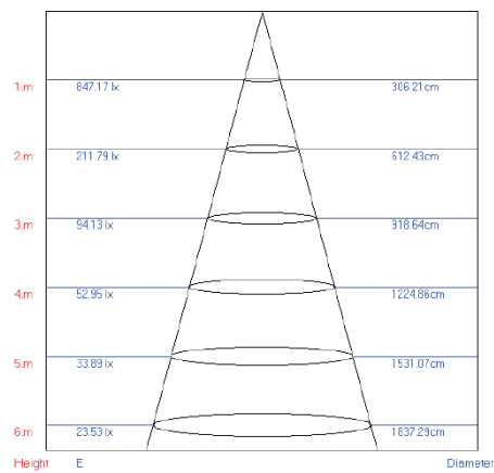
Lux-Distance Curve
